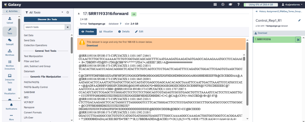
Figure 3. Forward read preview (Control_Rep1_R1) in FASTQ format following paired-end collection unzipping and extraction in Galaxy.
