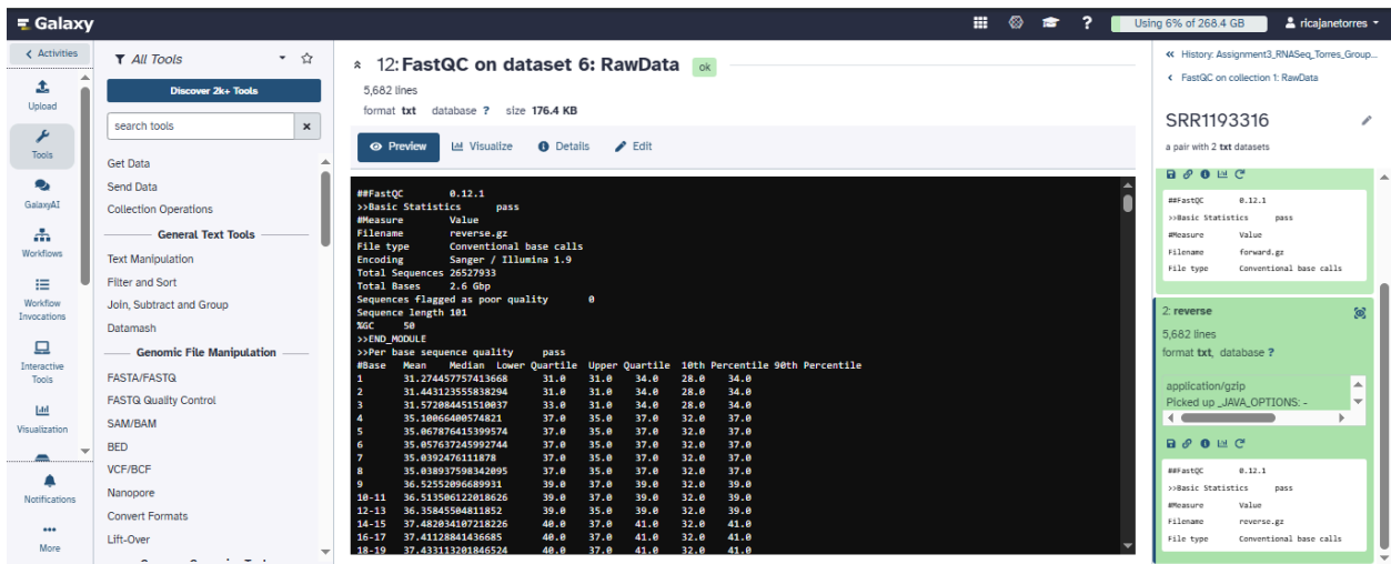
Figure 8. Raw Data Output of the FastQC Analysis for the Reverse Read (Control_Rep1_R2) Generated Using the FastQC Tool in Galaxy
