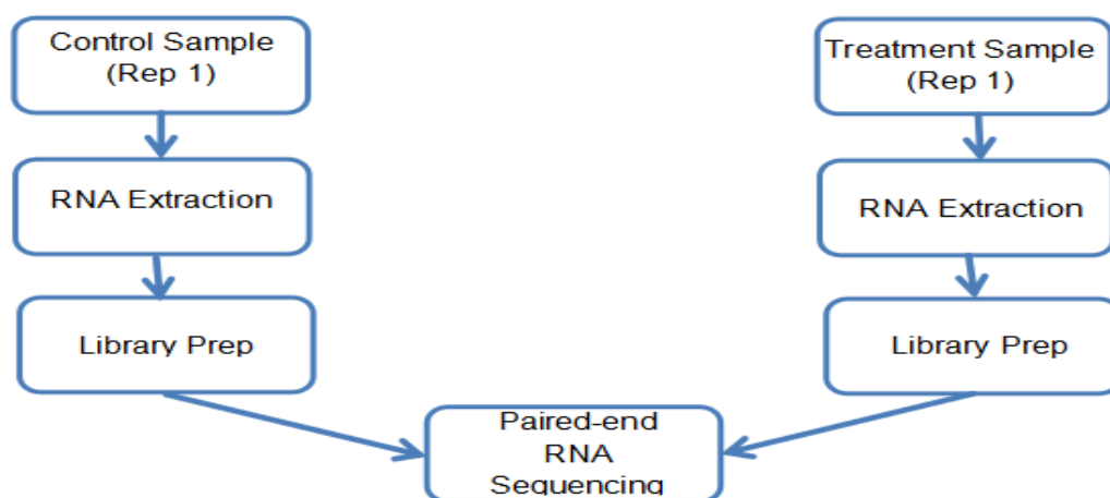
Figure 1. RNA-seq experimental design showing the steps from sample preparation to paired-end sequencing.
