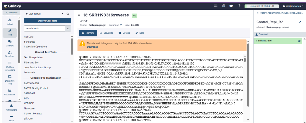
Figure 4. Reverse read preview (Control_Rep1_R2) in FASTQ format following paired-end collection unzipping and extraction in Galaxy.
