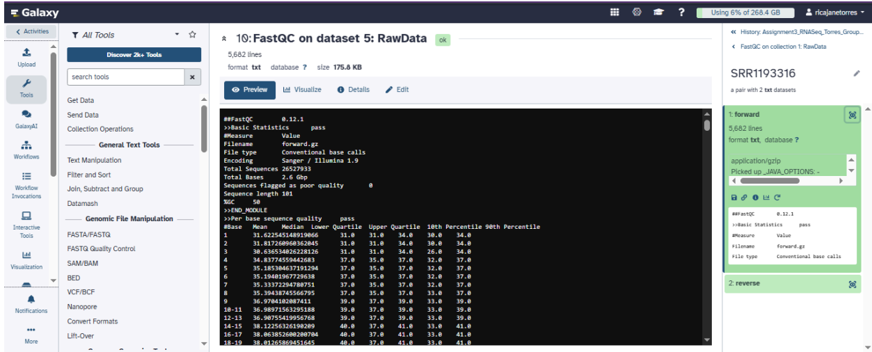
Figure 7. Raw Data Output of the FastQC Analysis for the Forward Read (Control_Rep1_R1) Generated Using the FastQC Tool in Galaxy
